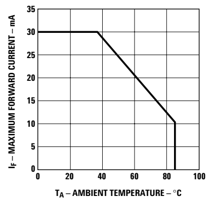
Figure 7. Maximum forward current vs. ambient temperature.
